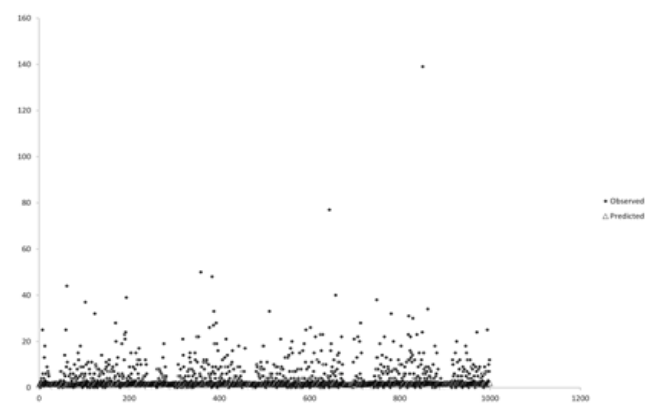
Figure 4: 1/100 random sample predicted by adjusted, standard error corrected linear model.
